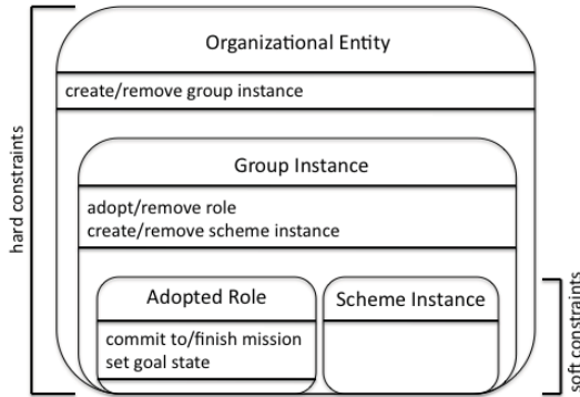
Figure 1: Participating in a MOISE + Organization
